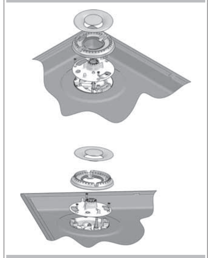
EXPLODED VIEW OF BURNER
